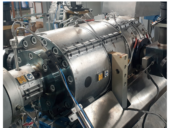
A detail of Tecnomatic's micro-pipe technology.
